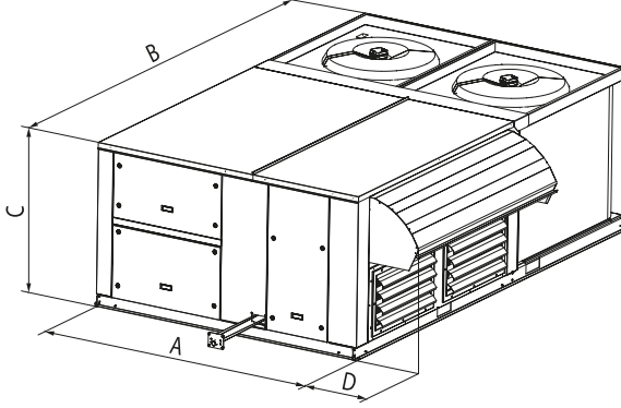
BALTIC SERİSİ - STANDART ROOFTOP CİHAZI
